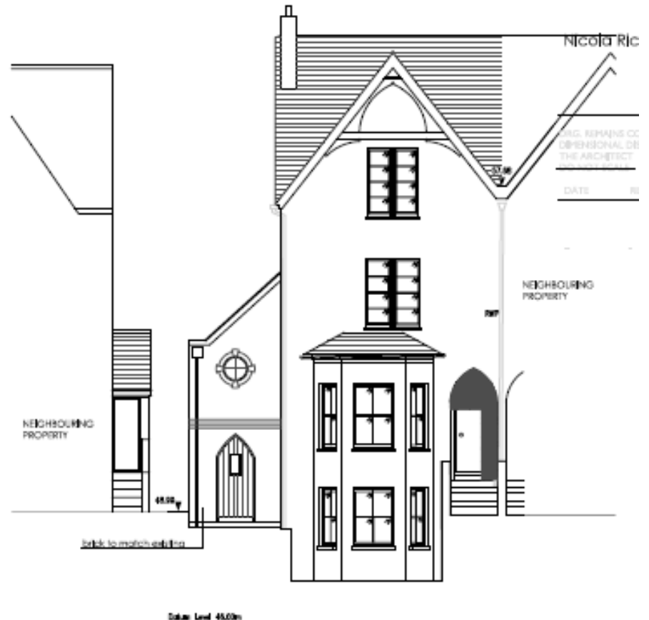
FRONT ELEVATION - NORTH
